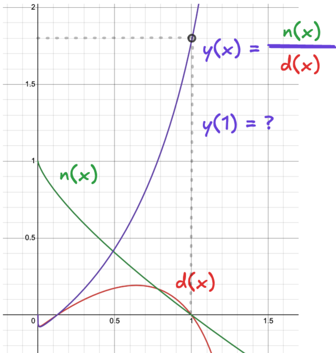
Figure 1: We have plotted the numerator and denominator separately in the ‘Varignon’ problem, and set a = 1
