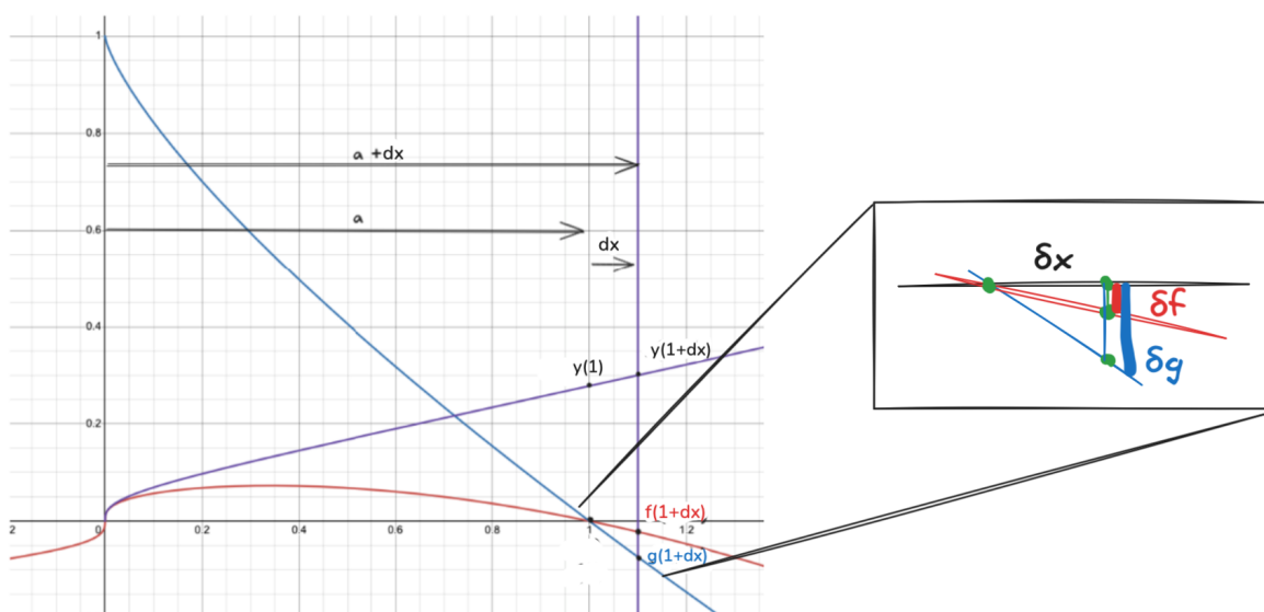
Figure 10: Since f(x) and g(x) intersect at x = 1 , we can replace their values with the infinitely small quantities df , dg , by applying Postulates I and II.
