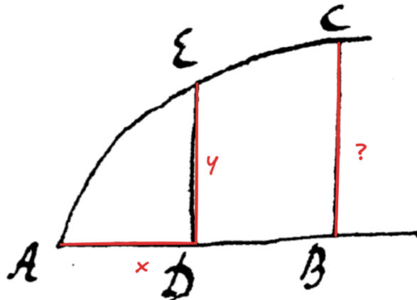
Figure 2: The initial set-up of the problem. BC is the length to be found. It is equal to a fraction, whose denominator and numerator are 0.
