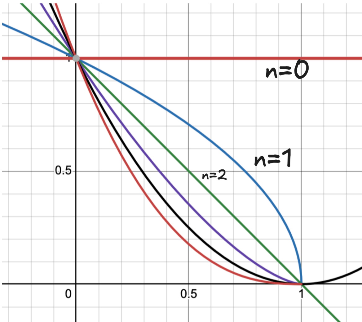
Figure 9: (1-x^2)^{\frac{n}{2}} plotted
