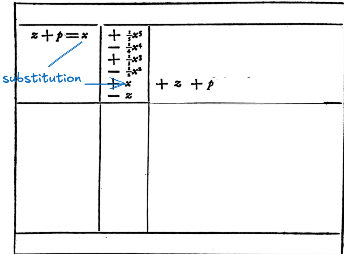
Figure 14: Using substitution z + p = x in one of the terms of the expansion of z(x)
