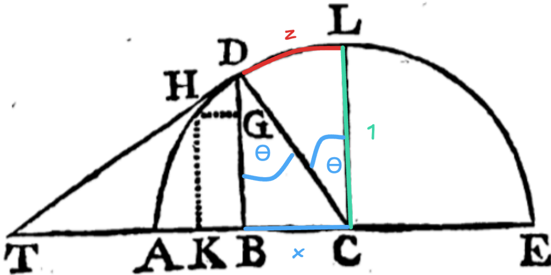
Figure 12: x = \sin(\theta) , and z = \theta
