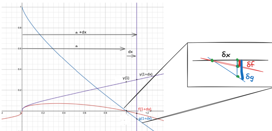
Figure 10: Since f(x) and g(x) intersect at x = 1 , we can replace their values with the infinitely small quantities df , dg , by applying Postulates I and II.
