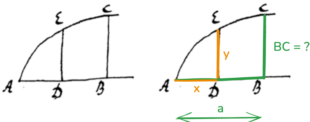
Figure 2: The initial set-up of the problem. BC is the length to be found. It is equal to a fraction, whose denominator and numerator are 0.
