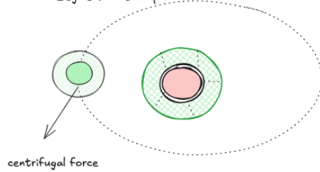
Analogous process happens for the planet; it flings off a ring which turns into a moon; Inner ring begins to break up
